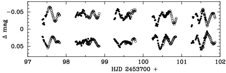
Figure 1: Light curves of the two mid B-type variables NSV 18451 (upper curve) and NSV 18457 (lower curve) from our campaign. The filled circles are SAAO data, the open circles are CTIO measurements. Complicated variability is evident.
