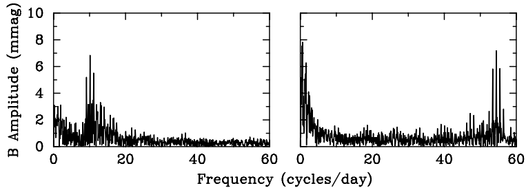
Figure 2: Amplitude spectra of the two \delta Scuti stars BVC 183 (left panel) and BVC 363 (right panel) in the field of NGC 3293 (B data from CTIO). The identification numbers are from Baume et al. (2003).
