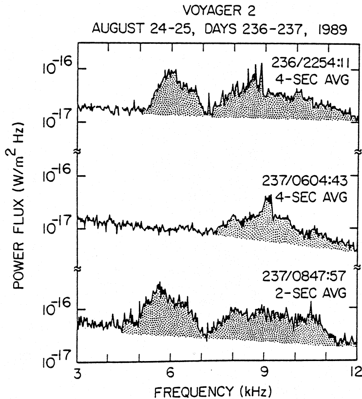
Figure 12: The spectrum of the low frequency radio emissions observed at Neptune [from Kurth et al., 1990a]. Like continuum radiation at the other planets, this emission shows both a diffuse background and narrowband emissions.
