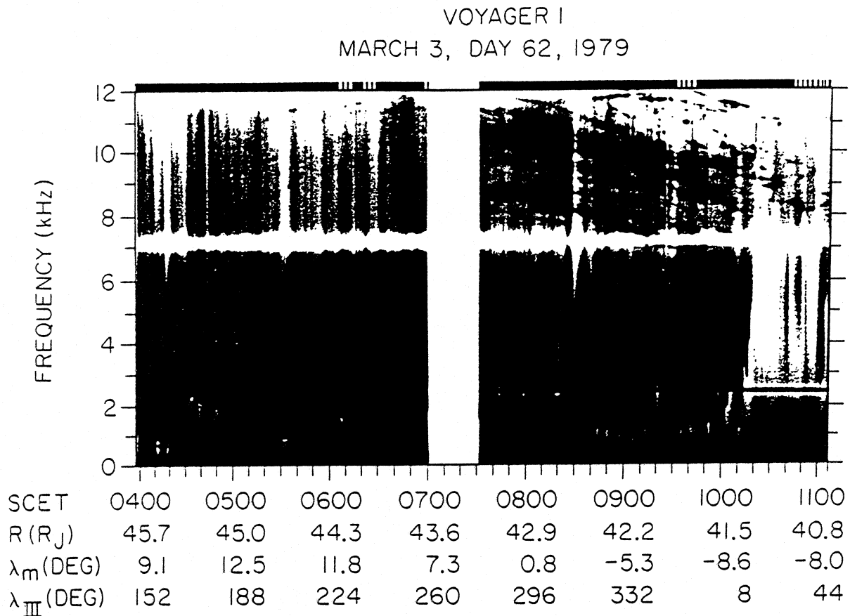
Figure 4: A spectacular family of drifting narrowband electromagnetic emissions from Jupiter. The time scale of the frequency variations is similar to that for the variations of geometrical parameters such as magnetic latitude and suggests beaming may be responsible for the frequency drifting.
