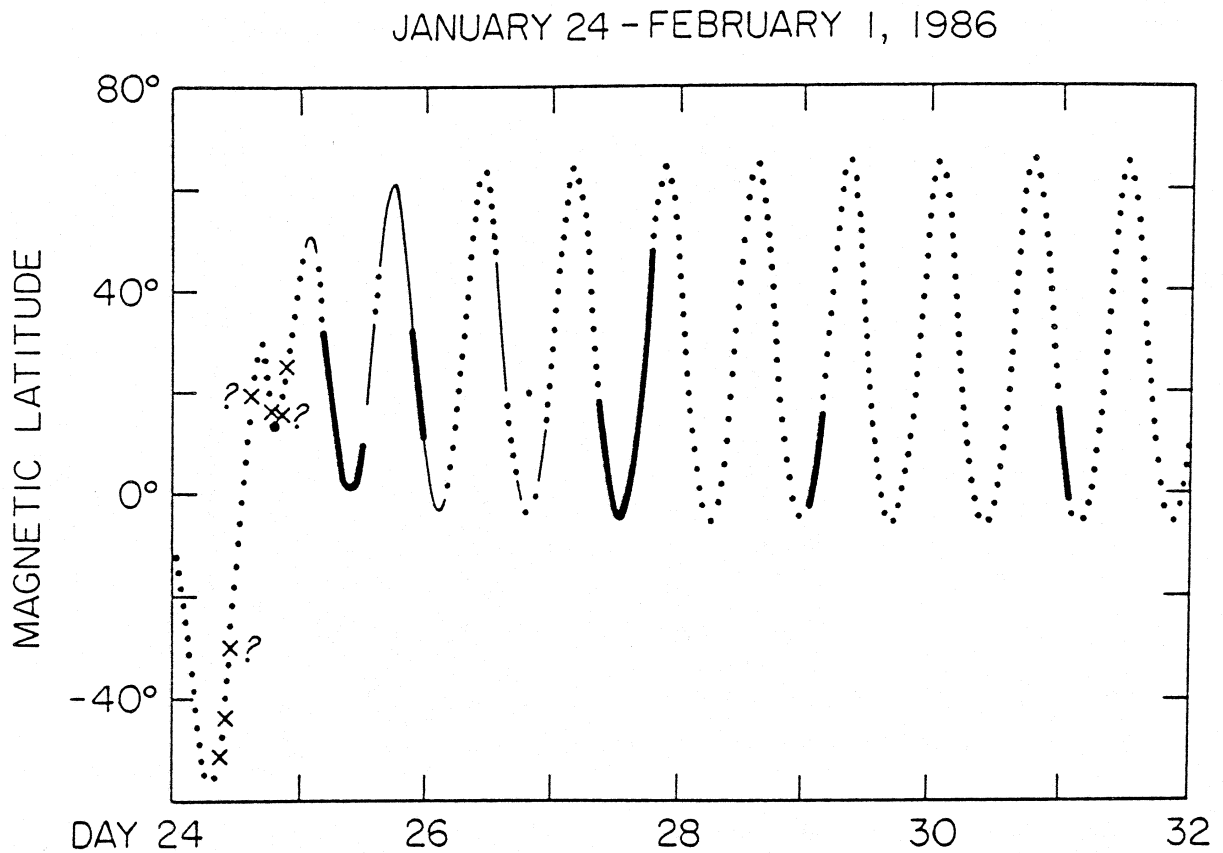
Figure 10: The trajectory of Voyager 2 in magnetic latitude as it departed from Uranus showing times when the sporadic narrowband emissions were detected [from Kurth et al., 1986]. This construction demonstrates that the bursty emissions are beamed towards low magnetic latitudes.
