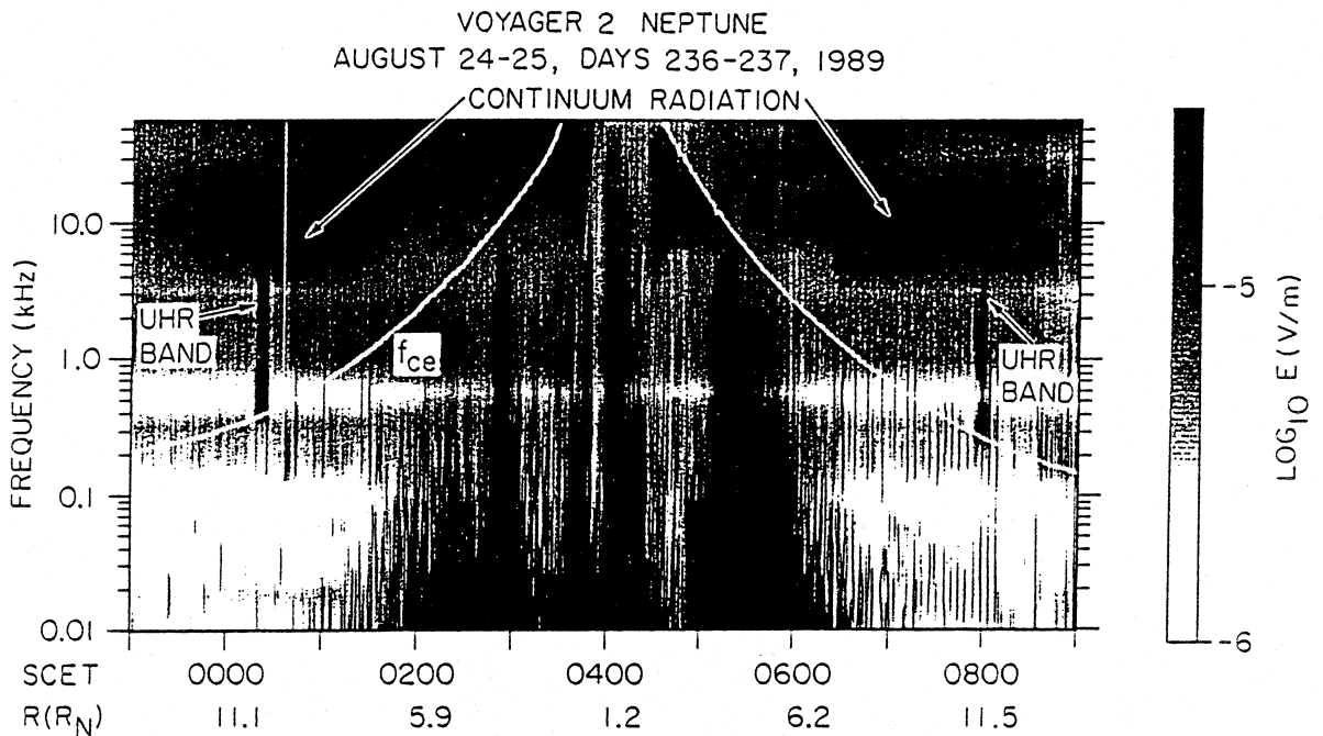
Figure 11: Low frequency radio and plasma wave observations at Neptune showing the escaping continuum radiation above about 5 kHz at larger radial distances and the electrostatic emissions (near 0030 and 0800 SCET) which are likely the source of the electromagnetic waves.
