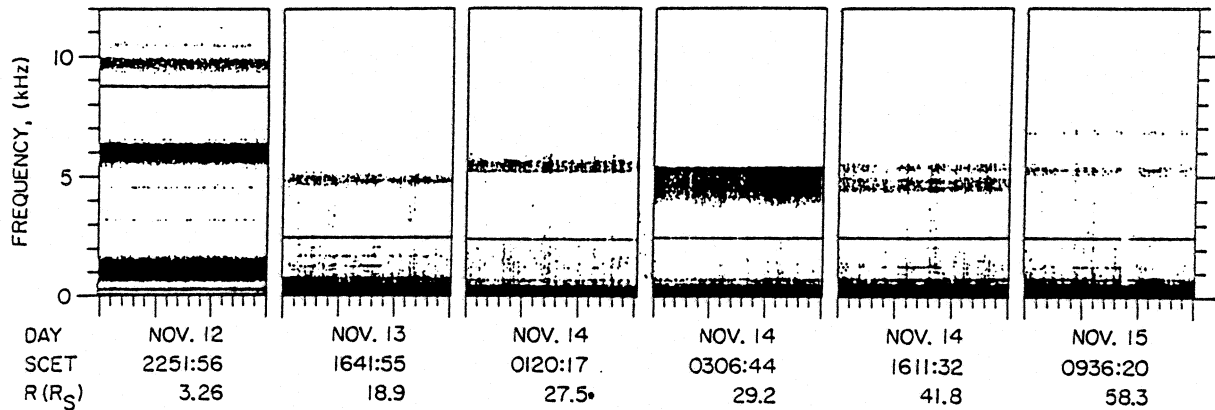
Figure 6: Examples of escaping narrowband electromagnetic bands observed by Voyager 1 near Saturn [from Gurnett et al., 1981].
