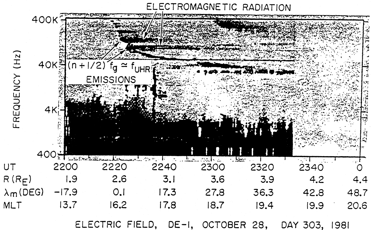
Figure 2: An excellent example of the generation of narrowband electromagnetic emissions from a series of upper hybrid bands at the terrestrial plasmopause. Since these waves are at frequencies well above the solar wind plasma frequency, they can escape from the magnetospheric cavity and form part of the escaping continuum radiation spectrum.
