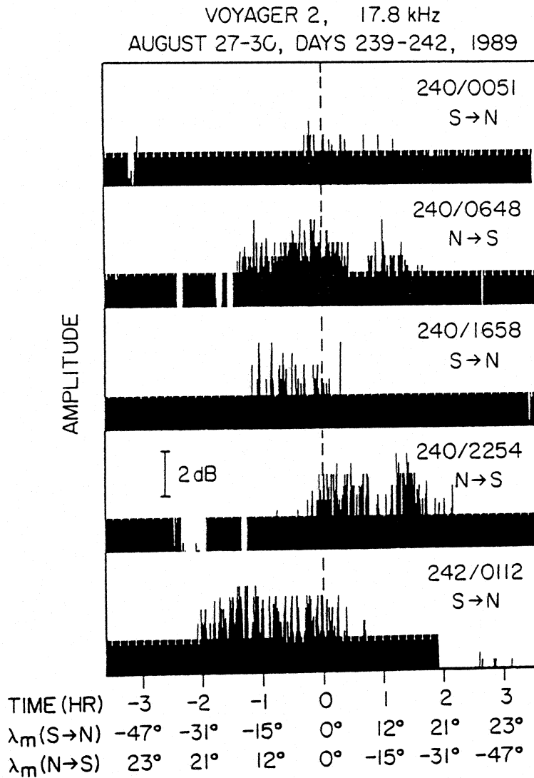
Figure 13: A series of low frequency radio emissions from Kurth et al. [1990a] showing their preference for low magnetic latitudes. While two of these sets of emissions suggest a local minimum in intensity near the magnetic equator as would be expected under the beaming prediction of the linear wave conversion mechanism, the evidence for the specific beaming predicted by the LWCM theory is not strong.
