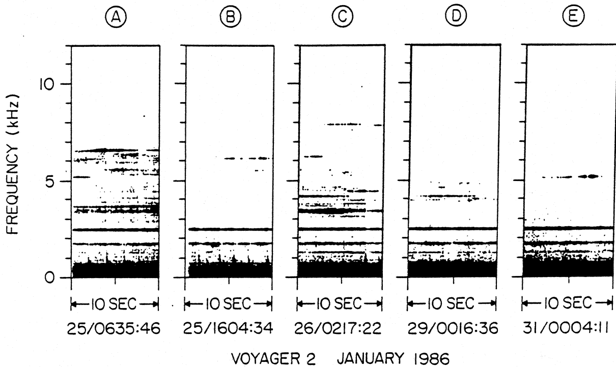
Figure 9: The sporadic narrowband radio emissions from Uranus [from Kurth et al., 1986]. It is not clear whether or not these emissions are the Uranian equivalent of escaping continuum radiation. The narrowband quality of the emissions is certainly suggestive, but the very bursty nature is not a typical characteristic of continuum radiation at other planets.
