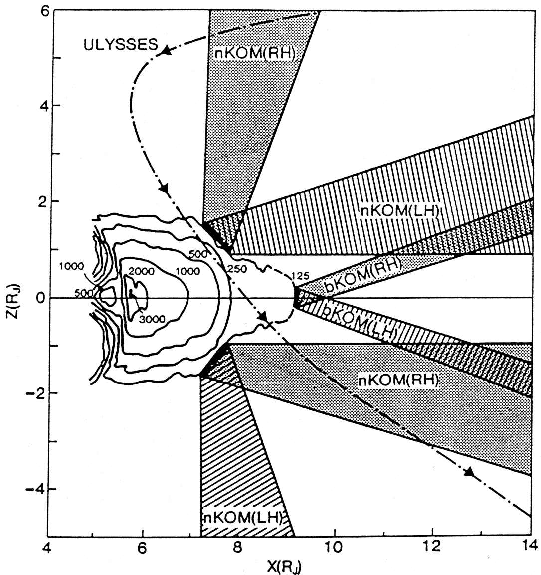
Figure 5: A model for Jovian narrowband and broadband kilometric radiation beaming proposed by Jones [1987, 1988]. Notice how details of the density model and the latitude of the source play a major role in determining the direction of the various beams.
