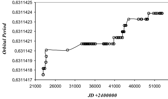
Figure 1: Orbital period variation of CG Cyg.
