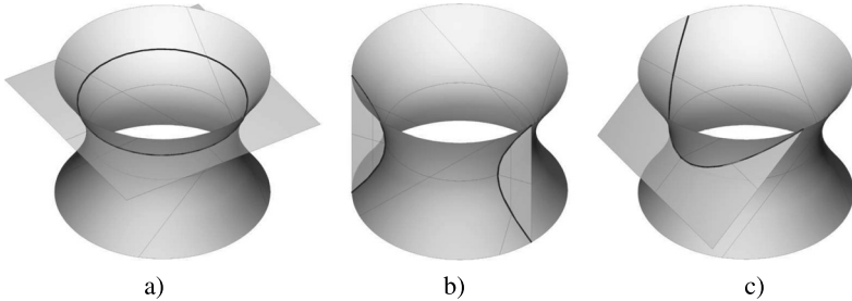
Fig. 5. The unit hyperboloid \mathcal{H} , canonical positions of a plane \pi and corresponding conic sections (Euclidean classification): a) space-like plane \pi_s and a ‘circle’ \mathcal{K}_s , b) time-like plane \pi_t and a ‘hyperbola’ \mathcal{K}_t , c) light-like plane \pi_l and a ‘parabola’ \mathcal{K}_l
