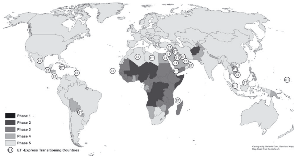
Figure 4: The development stages (phases) in the demographic transition process of the world's countries in the period 2005–10, with the 'express transitioning' countries marked
