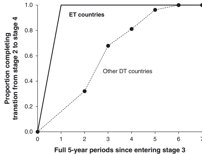
Figure 3: Tempo of the demographic transition (DT) from phase 2 to phase 4 of the 'express transitioning' (ET) countries and the other countries that underwent the demographic transition between 1950 and 2010
