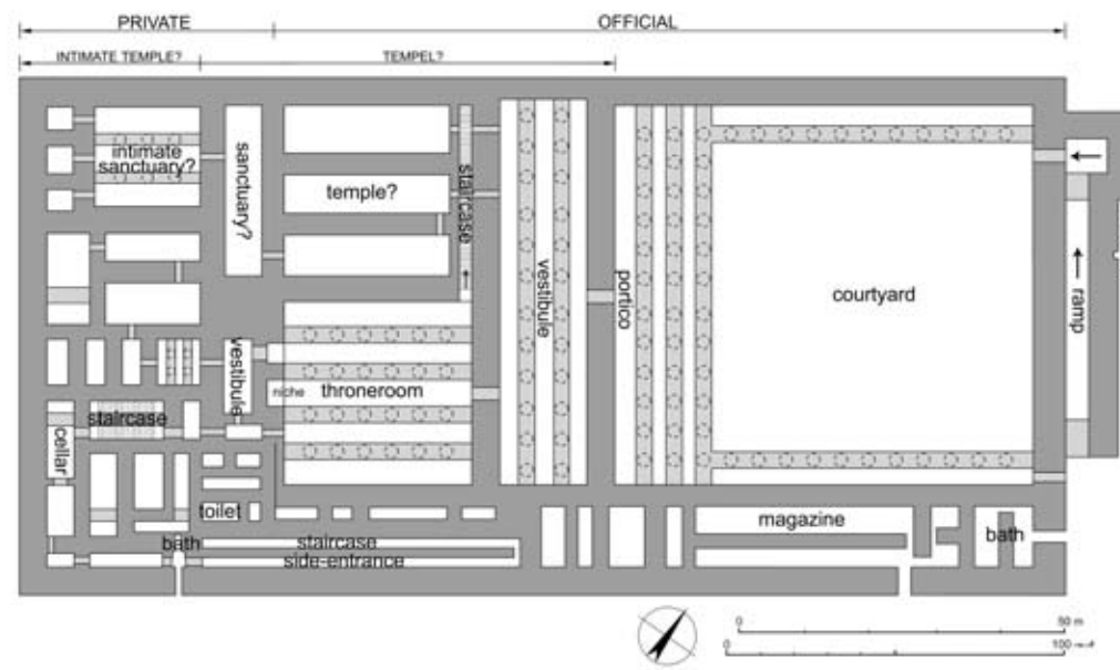
Fig. 29 Palace G of the Tuthmosid Period, reconstruction
