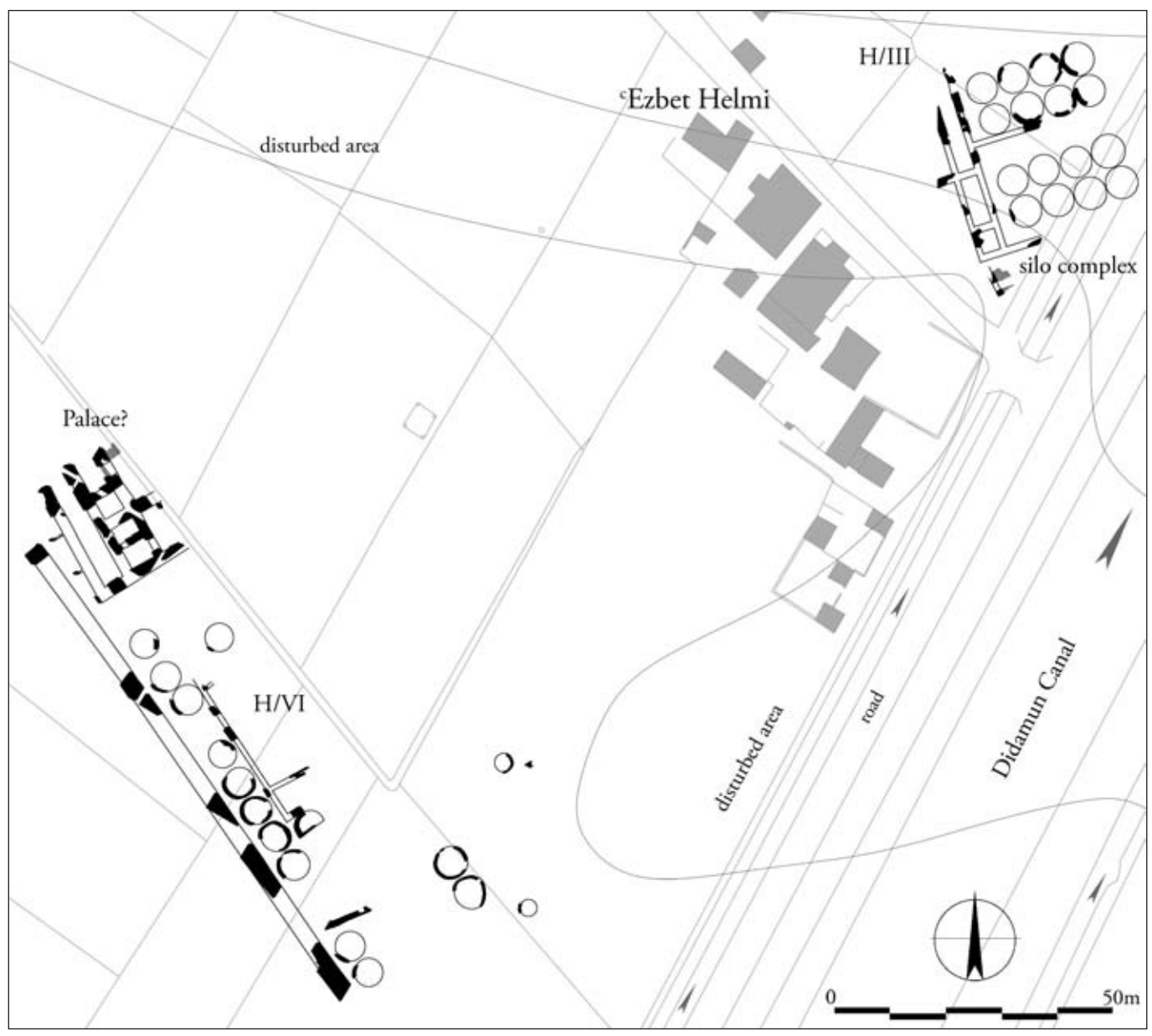
Fig. 27 Storage facilities and a small palace of the early 18 th Dynasty in Area H, Ph. D/1.2
