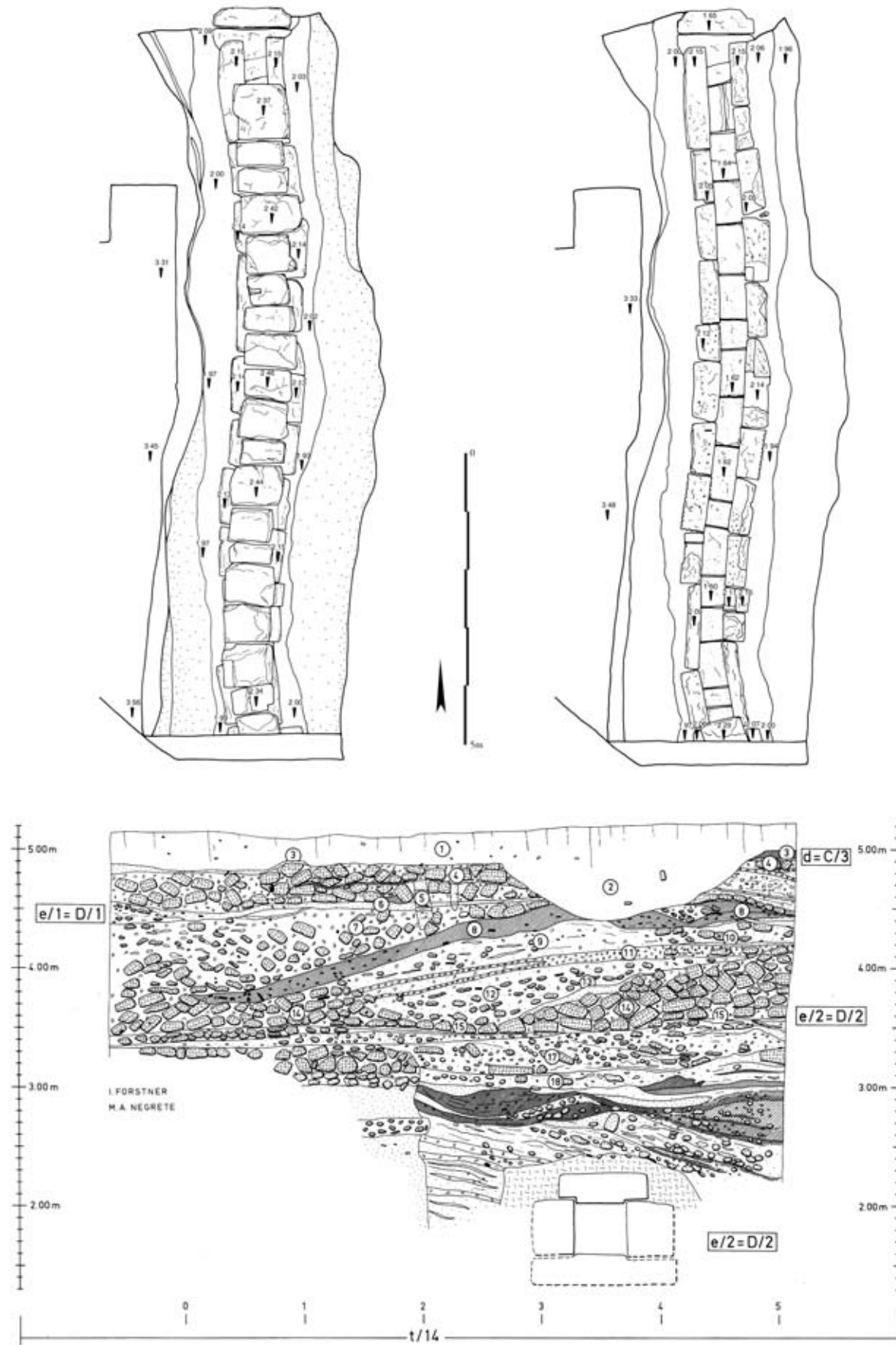
Fig. 26b Water supply systems of the Palace compound of the Hyksos Period in Area H/III, Ph. D/2
