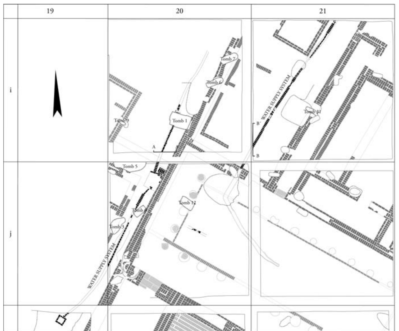
0 20m TELL el-DABSA F/1 STR. d/1-1
