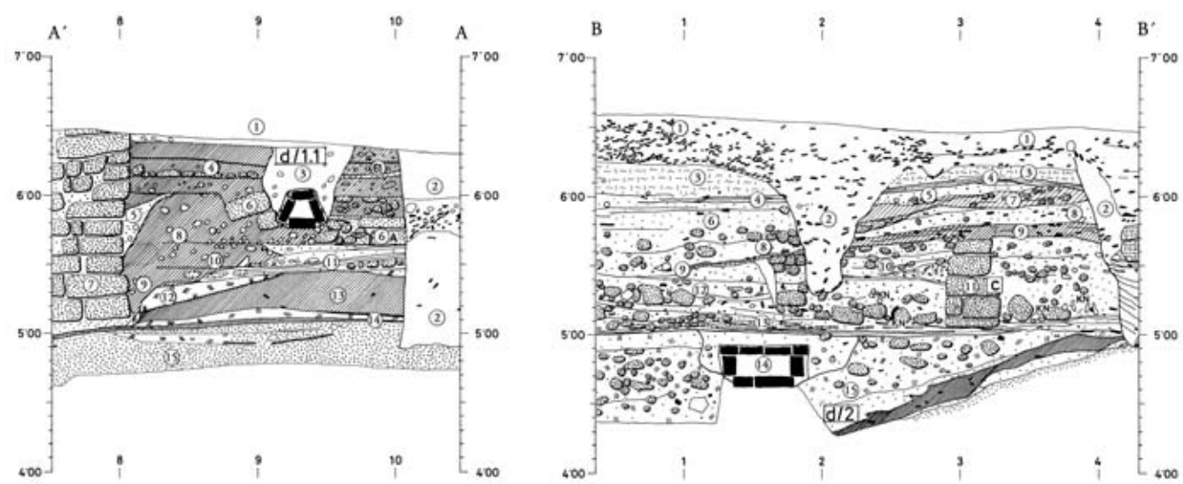
Fig. 26a Water supply systems of the mansion in Area F, Ph. G/4
