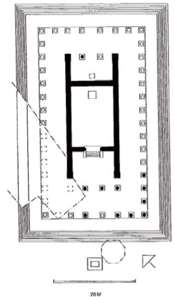
Abb. 3: Oktostyler Pseudodipteros (© C. Coockson in: BENNETT 2003, 7 Abb. 1.4)
